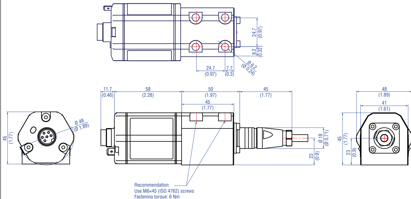
Fig. 4: Temposonics® RD5 sensor electronics & mounting block
