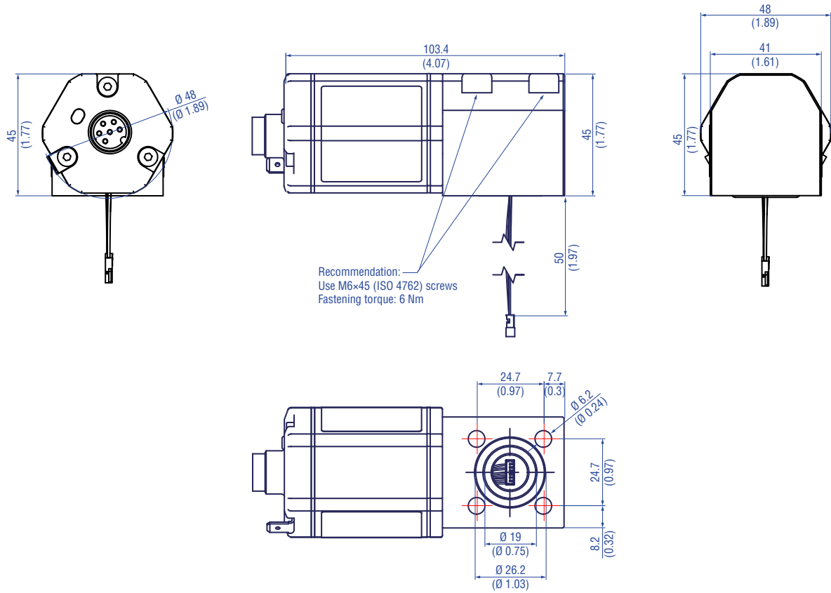
Fig. 6: Temposonics® RD5 sensor electronics & mounting block
